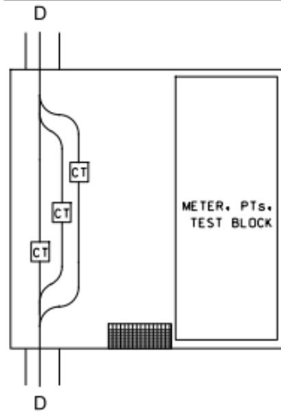
CABINET LAYOUT EXIT AND ENTRY POINTS: D TO D
