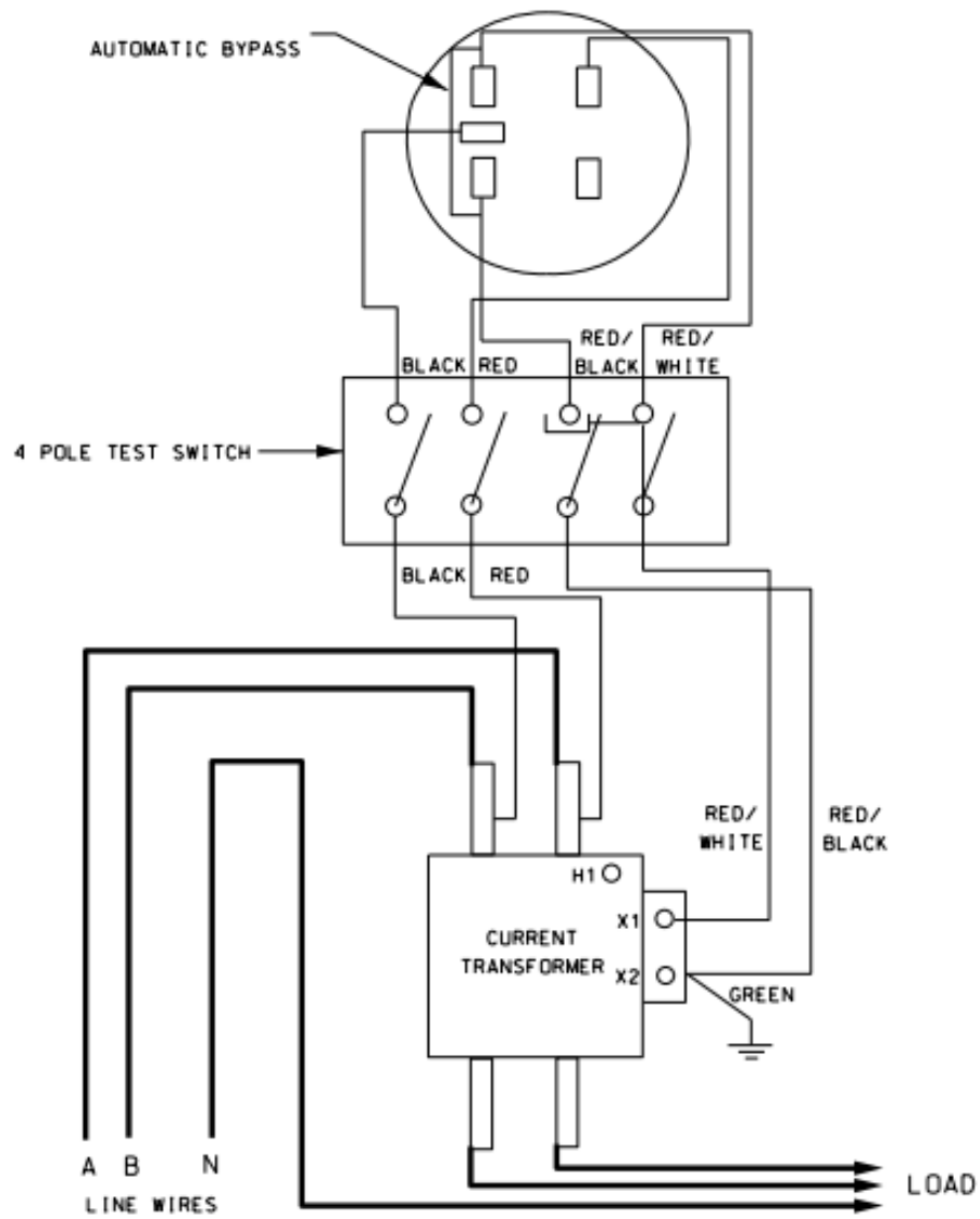
WIRING DIAGRAM
