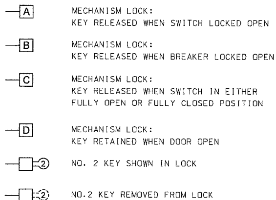
SKETCH 1 (A-1) TYPICAL SINGLE LINE DIAGRAM LEGEND
