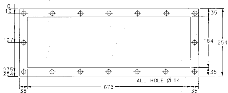
MOUNTING PLATE GASKET (3 mm THICK)
